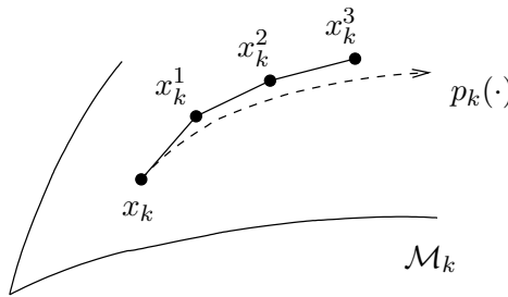
Fig. 18.2. Piecewise linear search
