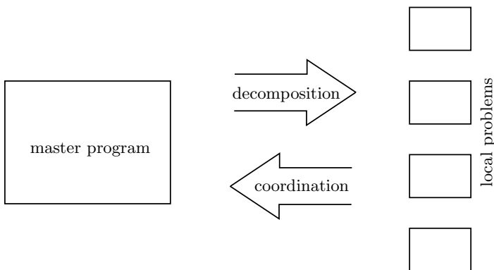
Fig. 11.1. Decomposition/coordination
