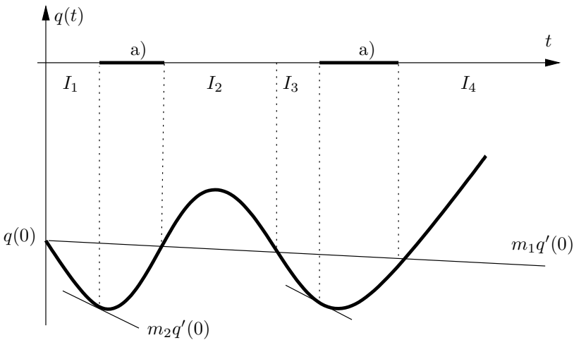
Fig. 3.2. Wolfe's rule
