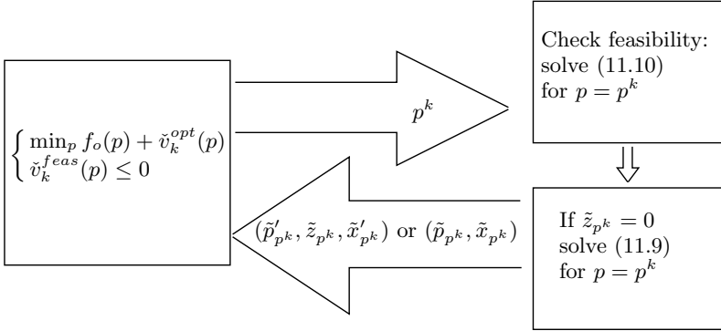
Fig. 11.4. Benders decomposition
