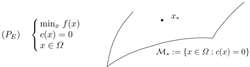
Fig. 14.1. Problem (P_E) and its feasible set
